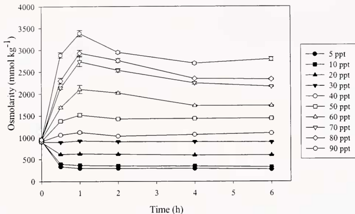
Figure 5. Mean ( \pm SE) osmotic concentration of the perivittelline fluid at 0, 0.5, 1, 2, 4, and 6 h after exposure to salinities ranging from 5 to 90 ppt.
